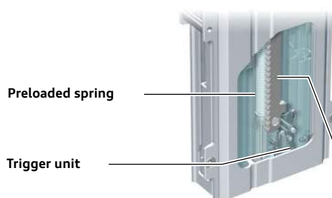
Latching mechanism
